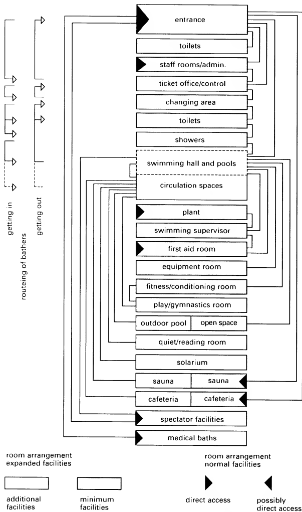
① Indoor swimming pool: organisation of spaces
